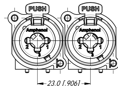
MIN MOUNTING PITCH
