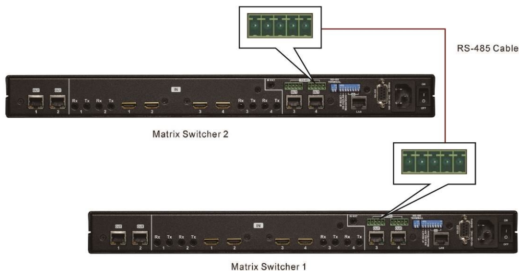
Figure 6-14 RS-485 Connection for HIT-HDMI4K2KCAT5-X444
