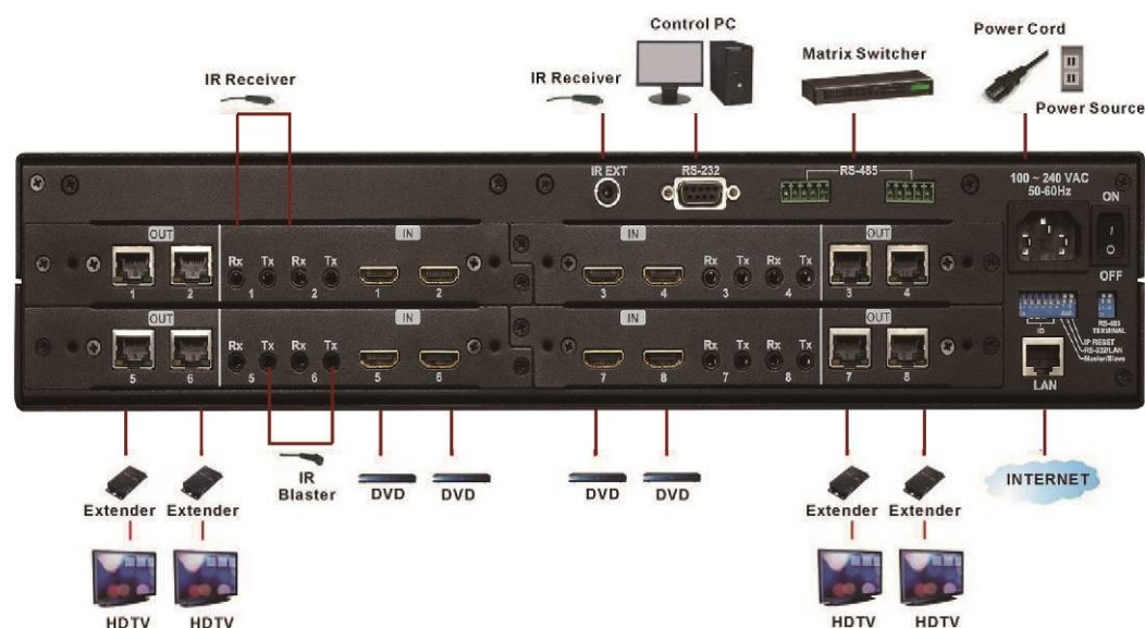
Figure 6-2 HIT-HDMI4K2KCAT5-X848 Connections
