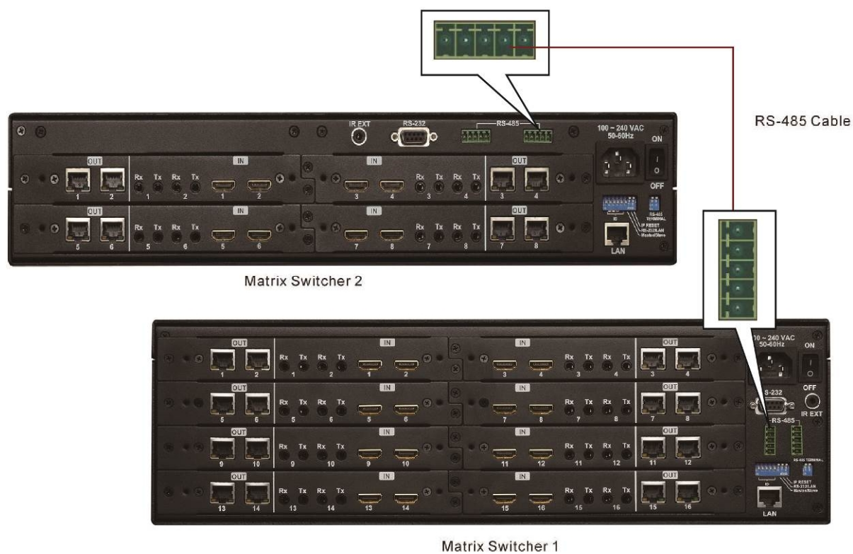
Figure 6-17 RS-485 Connection for HIT-HDMI4K2KCAT5-X848 and HIT-HDMI4K2KCAT5-X16416
