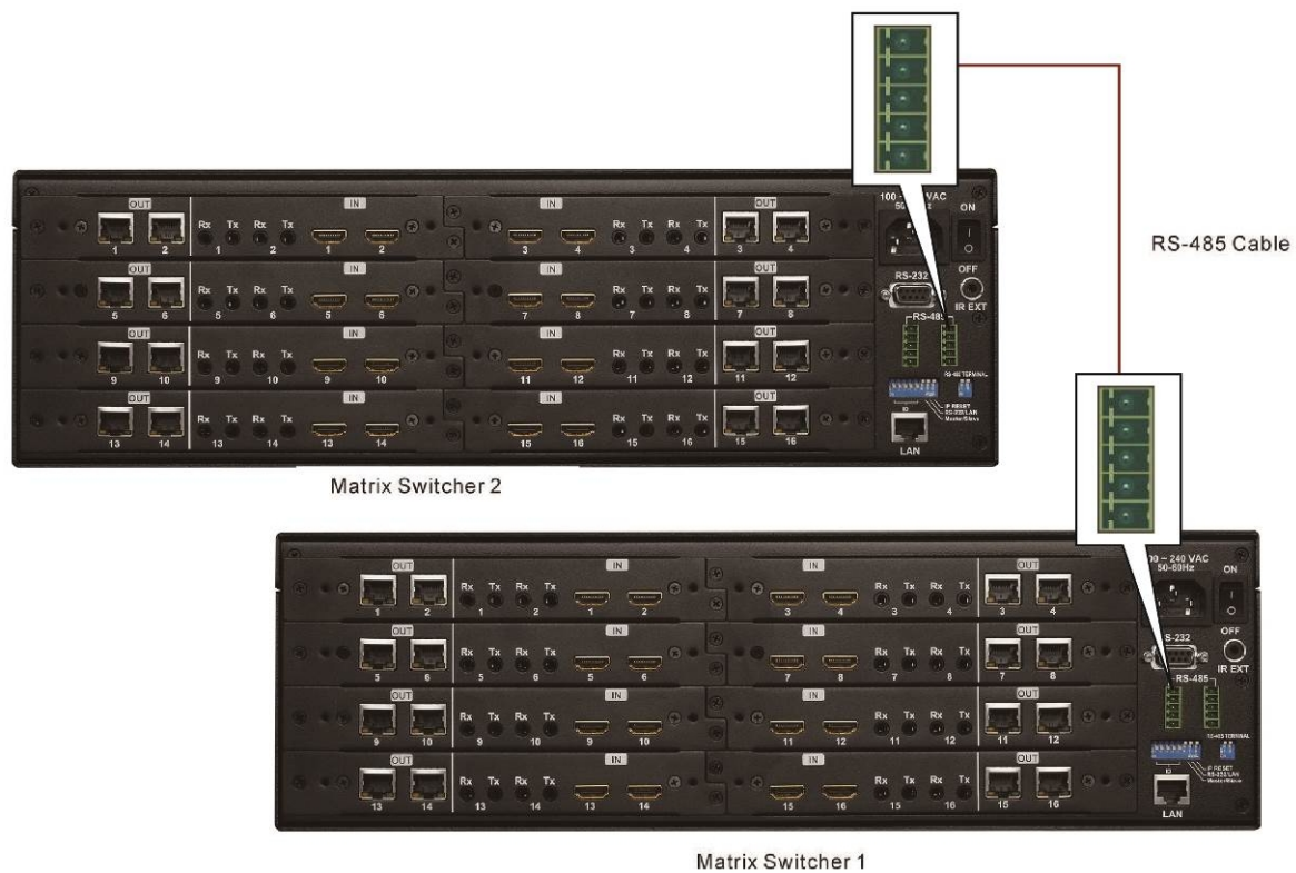
Figure 6-16 RS-485 Connection for HIT-HDMI4K2KCAT5-X16416
