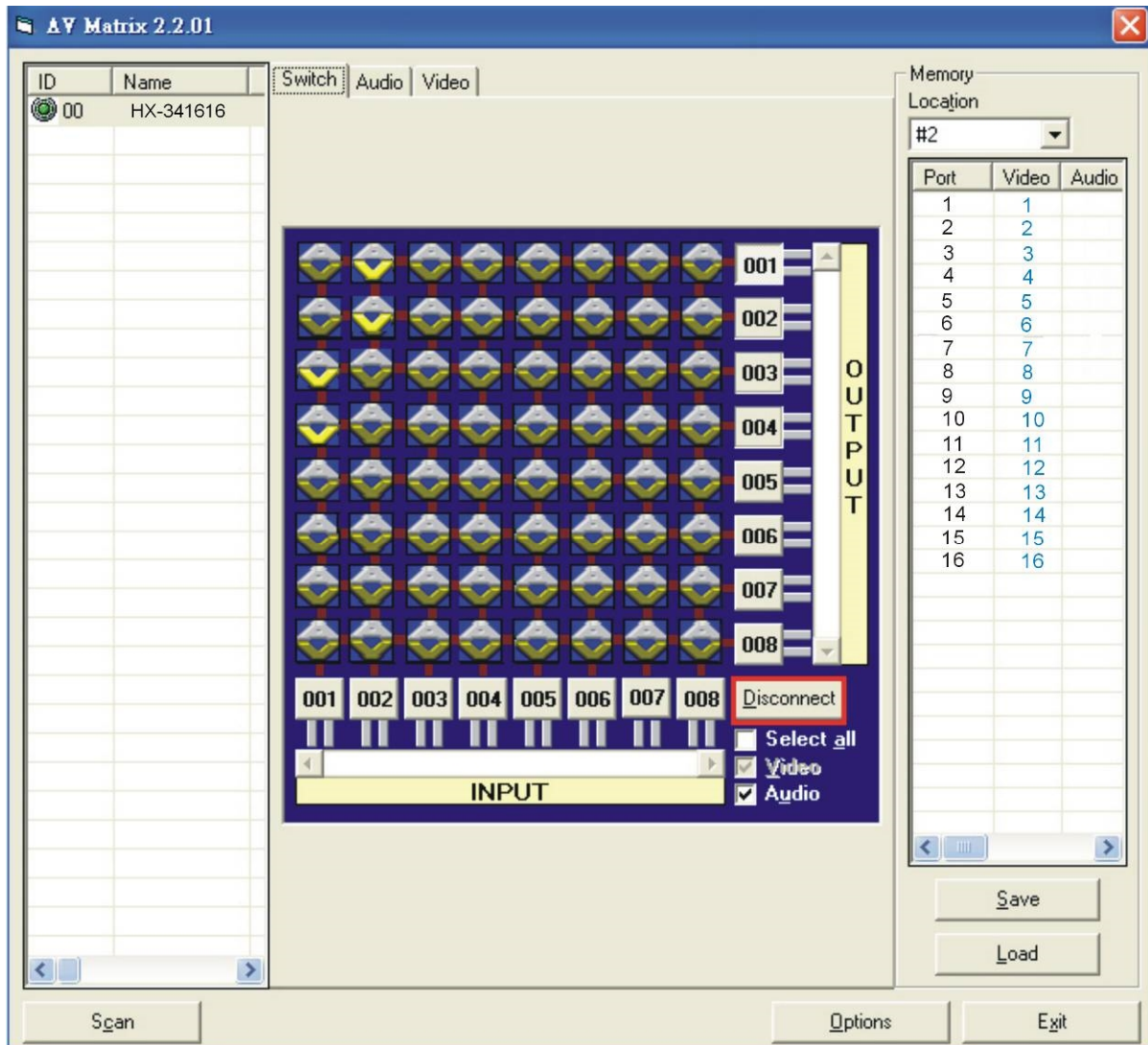
Figure 7-4 Disconnect Function Key (a) for HIT-HDMI4K2KCAT5-X16416 Reference
