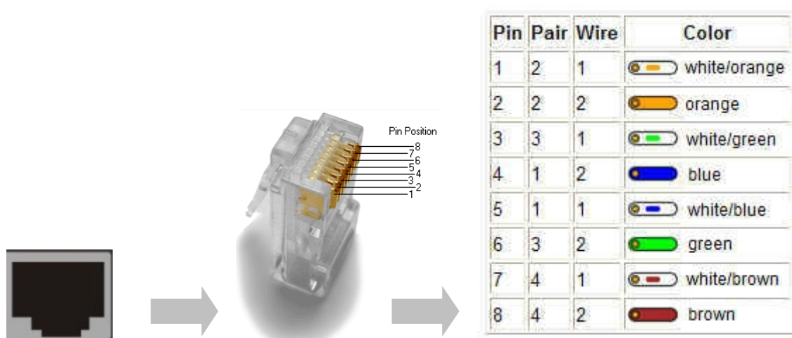
Figure 6-19 RJ45 Connector
