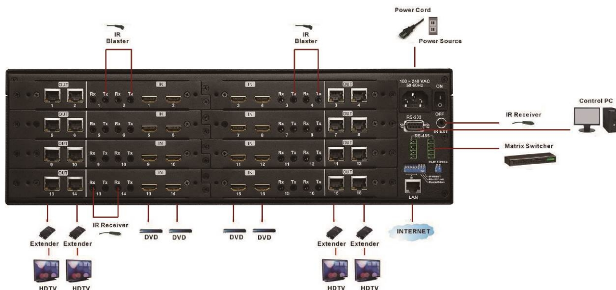
Figure 6-3 HIT-HDMI4K2KCAT5-X16416 Connections
