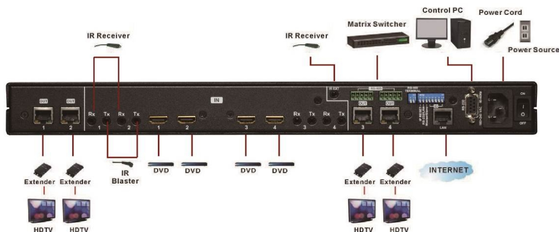
Figure 6-1 HIT-HDMI4K2KCAT5-X444 Connections
