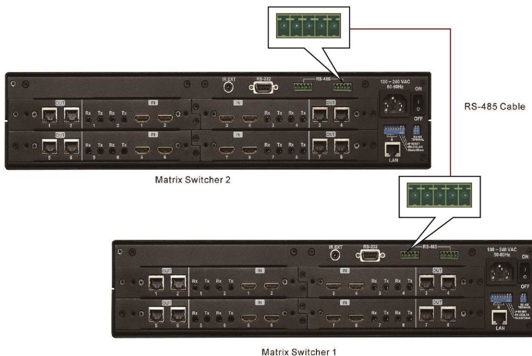
Figure 6-15 RS-485 Connection for HIT-HDMI4K2KCAT5-X848
