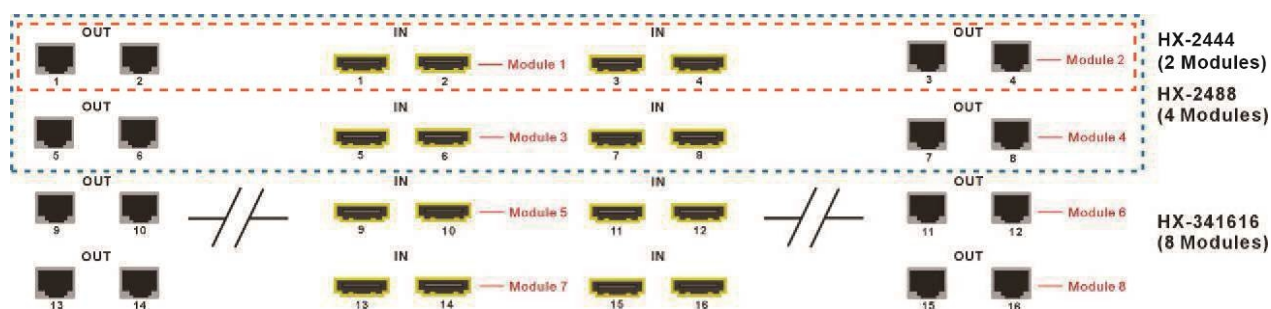
Figure 6-4 Modules Deployment
